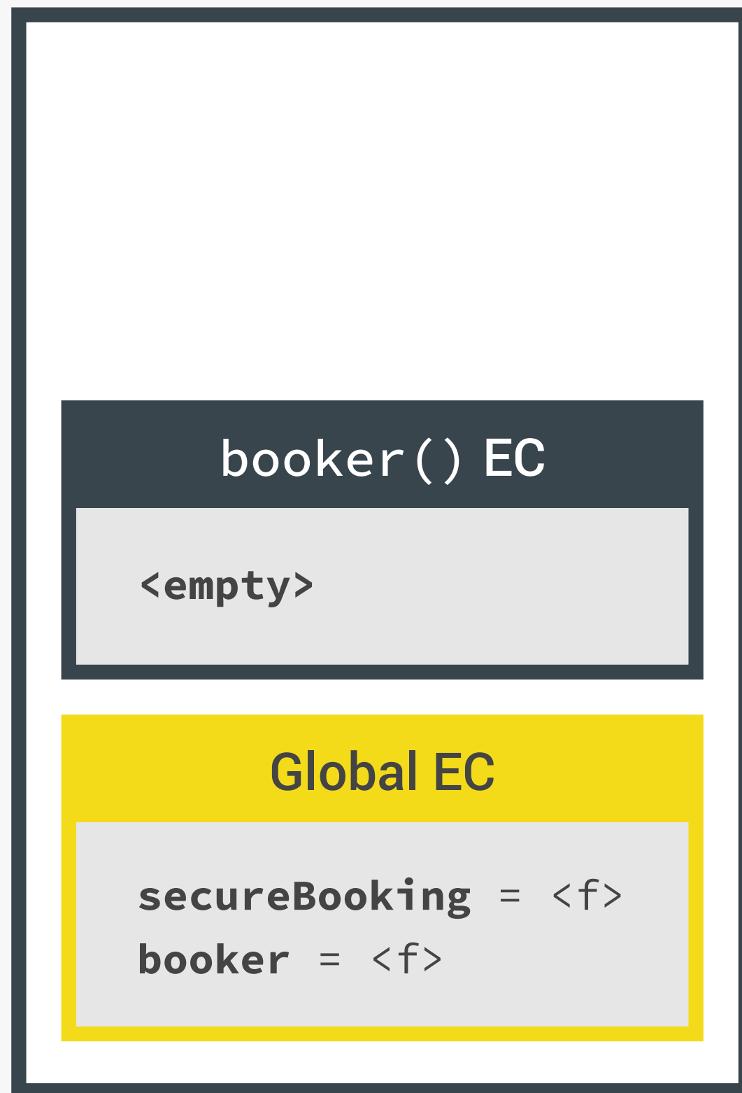
CALL STACK
